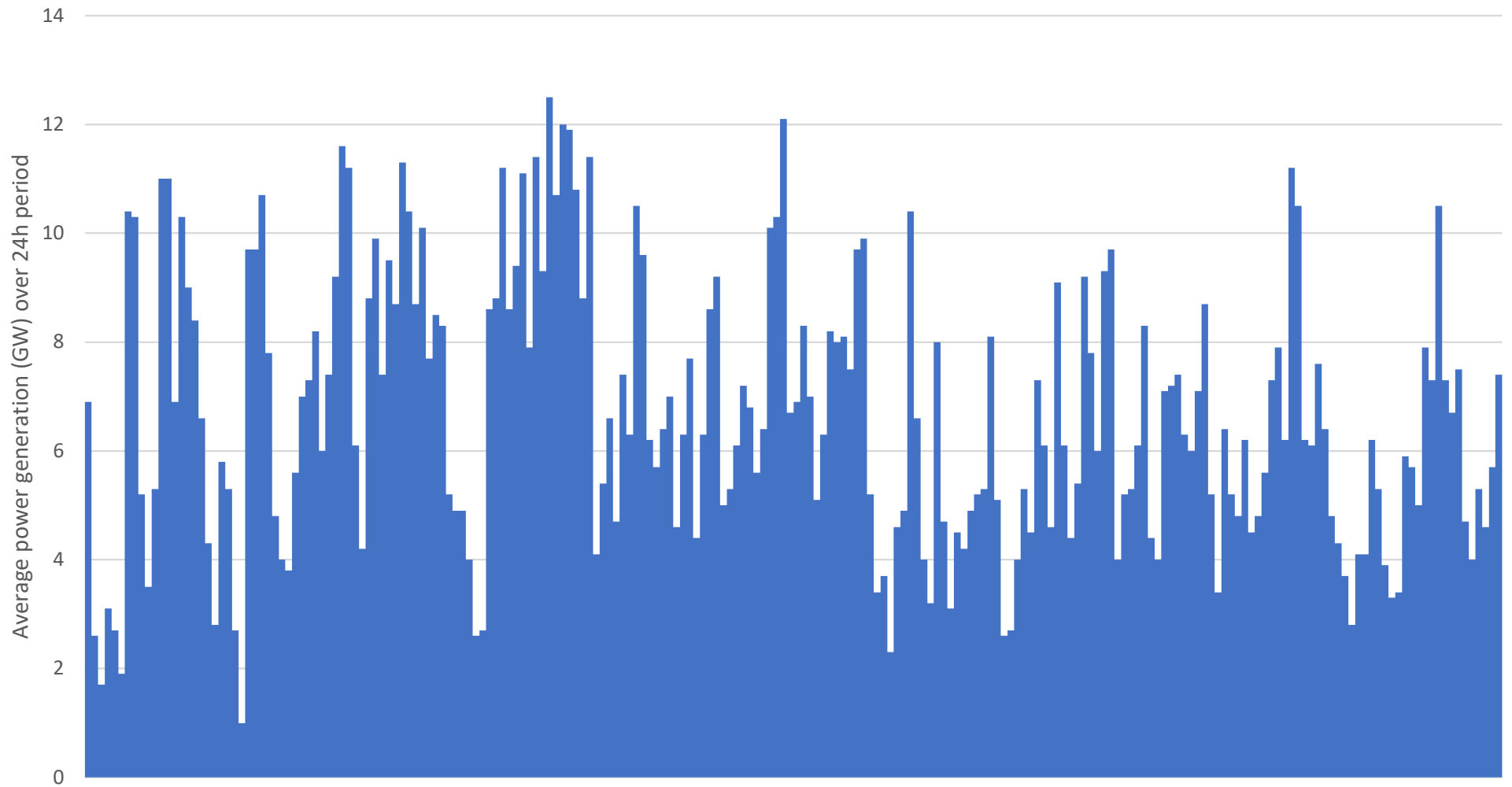
Electricity from wind & solar PV (2019)
